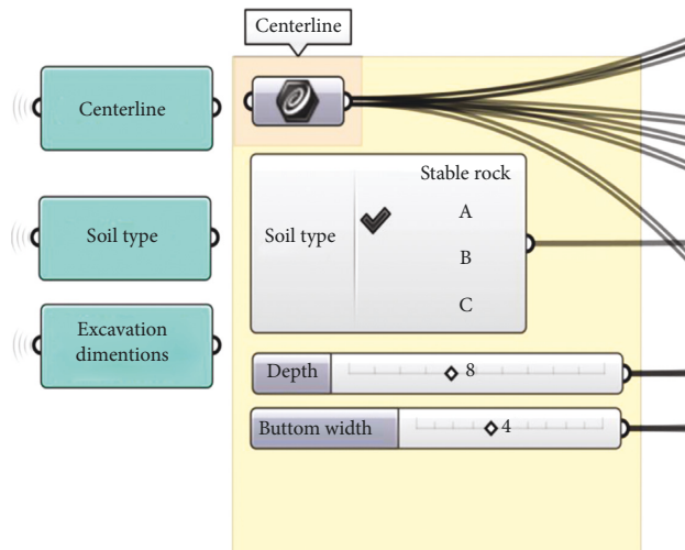
FIGURE 6: Soil classification and dimension constraint algorithm.
