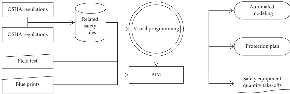
FIGURE 1: Conceptual framework for automated safety excavation modeling approach.
