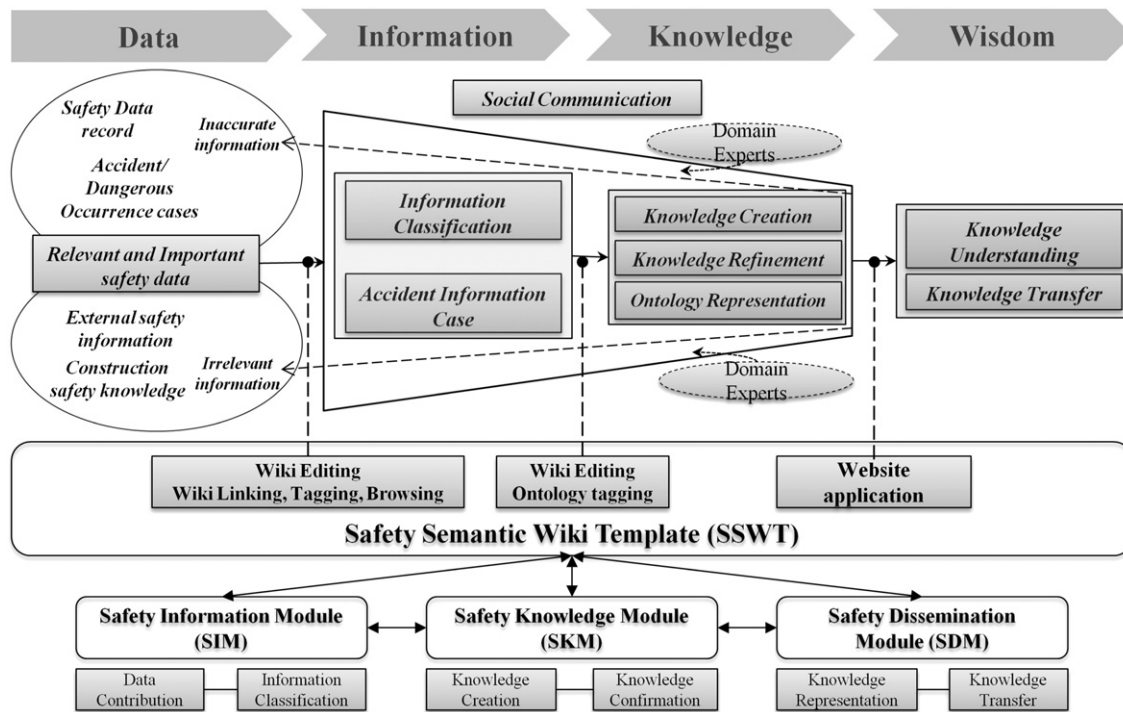
Fig. 1. The disintermediation process of SNSS.
